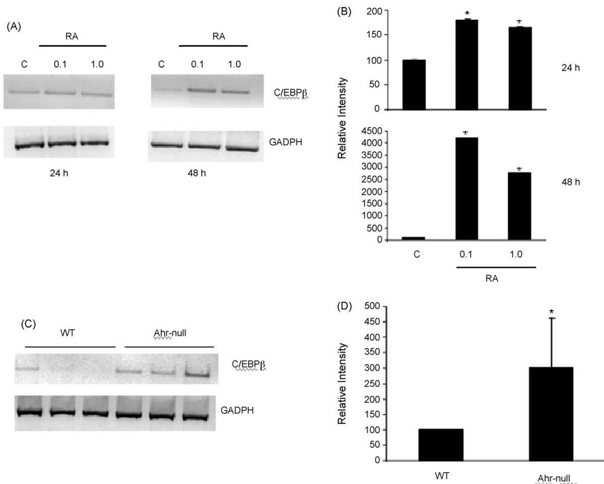
Fig. 7 – Effect of RA treatment on C/EBPβ mRNA levels. (A) Hepa-1 cells were treated with 0.1 or 1.0 μM of RA for 24 or 48 h, C/EBPβ mRNA levels were determined by RT-PCR, the relative intensity of the signal was quantified (B). (C) Liver RNA, isolated from Ahr-null and wild-type mice, was subjected to RT-PCR analysis, and the relative intensity of the signal was quantified (D). Signals were normalized relative to GADPH. Data are presented as the mean levels of expression \pm SD of triplicates, *p < 0.05 .
