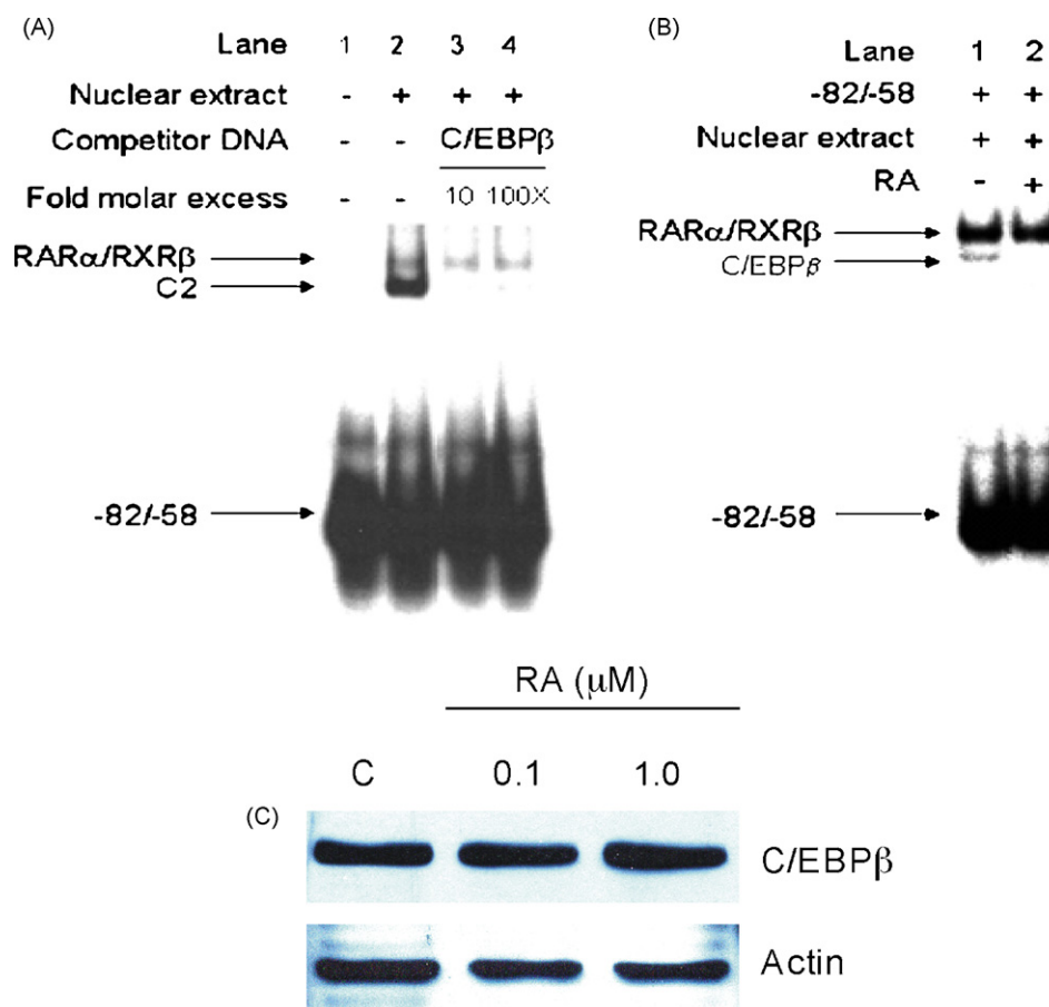
Fig. 6 – (A) Competitive EMSA to identify the CCAAT box binding protein. Unlabeled oligonucleotide containing the consensus sequence of C/EBPβ was incubated with Hepa-1 nuclear extract for 30 min at the indicated molar excess prior to addition of the –82/–58 bp labeled probe. Arrows identify the shifted bands and the unbound radiolabeled probe. (B) Effect of RA on C/EBPβ binding. Nuclear extracts from RA-treated (1.0 μM RA, 72 h) Hepa-1 cells were incubated with radiolabeled mouse –82/–58 bp probe (lane 2) and analyzed by EMSA. Arrows identify the shifted bands and the unbound radiolabeled probe. (C) Effect of RA treatment on C/EBPβ protein levels. Hepa-1 cells were treated with 0.1 or 1.0 μM of RA for 72 h and cell lysates were incubated with C/EBPβ antibody. C/EBPβ protein levels were determined as described in Section 2. A representative set of data from two independent experiments is shown.
