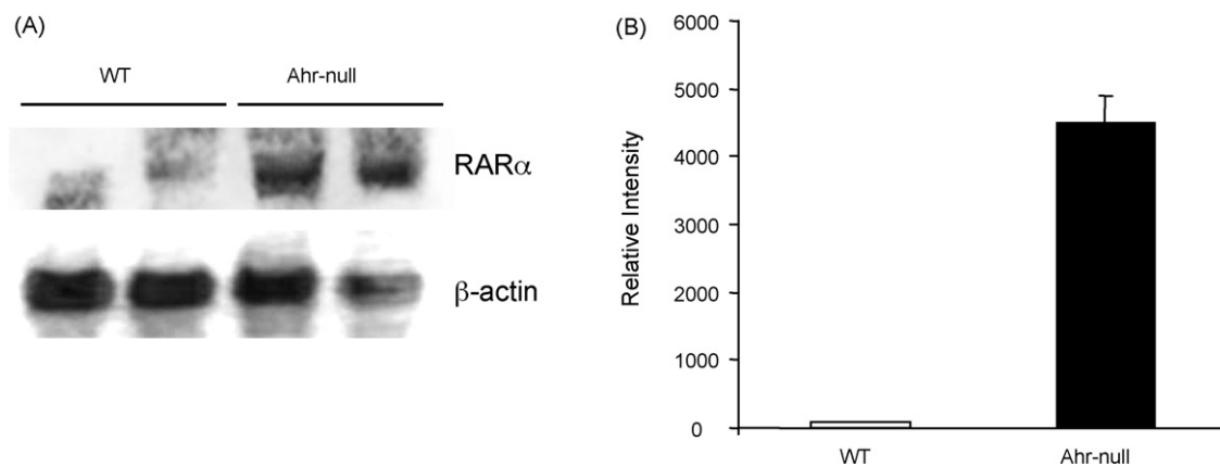
Fig. 8 – Northern blot analysis of RARα. (A) Liver total RNA, isolated from Ahr-null and wild-type mice, was subjected to Northern blot analysis. Mouse actin mRNA was used to verify integrity. (B) Following hybridization, the membrane was exposed to phosphor screen, and the signal was quantified. Data are presented as the mean levels of expression \pm SD, n = 3 .
