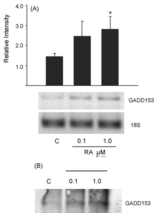
Fig. 9 – (A) Effect of RA treatment on GADD-153 mRNA levels. Hepa-1 cells were treated with 0.1 or 1.0 \mu M of RA for 24 h and GADD-153 mRNA levels were determined by RT-PCR, and the relative intensity of the signal was quantified. Data are presented as the mean levels of expression \pm SD of triplicates, * p < 0.05. (B)
