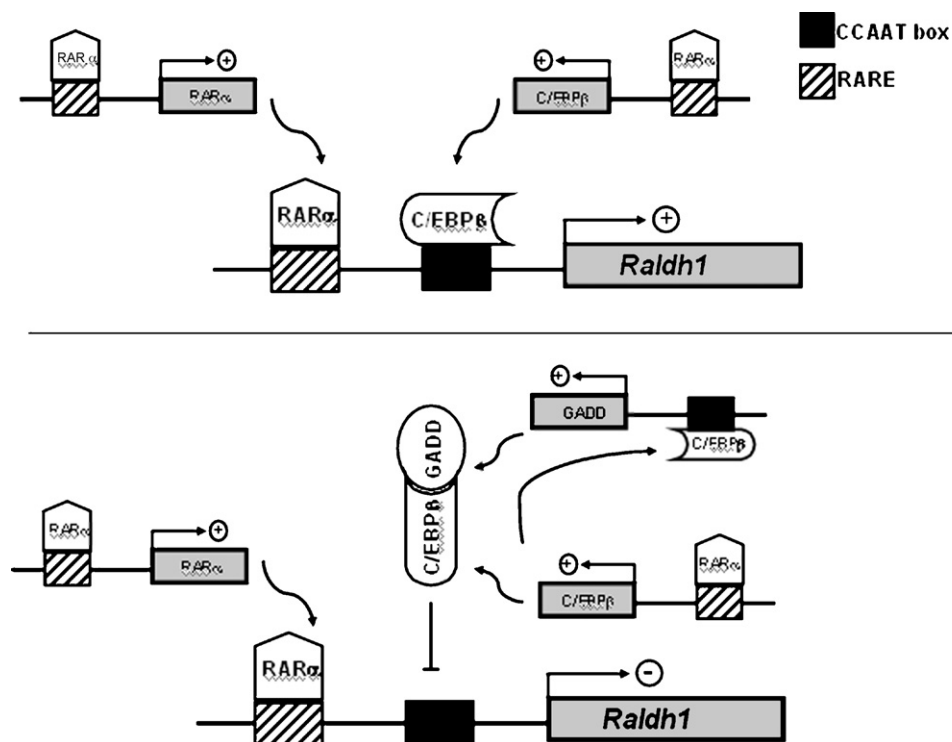
Fig. 10 – Model of autoregulation of the Raldh1 gene promoter by heterodimerization of GADD153 and C/EBPβ. At low RA concentrations RARα and C/EBPβ transactivate the Raldh1 promoter (top panel). When RA levels increase, RARα transactivate the C/EBPβ promoter increasing the C/EBPβ abundance resulting in an increase of GADD153 amount and the formation of GADD153–C/EBPβ heterodimers (lower panel).
