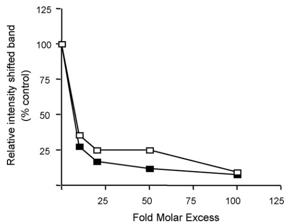
Fig. 5 – Competitive binding analysis of the RARα/RXRβ complex to Raldh1 gene promoter. Nuclear extracts were incubated with radiolabeled mouse –82/–58 bp probe and varying amounts of unlabeled –82/–58 bp (open squares) and consensus RARE (closed squares) probes. Following EMSA, the intensity of shifted band, identified as a RARα/RXRβ DNA complex, was quantitated by densitometry. A representative set of data from two independent experiments is shown.
