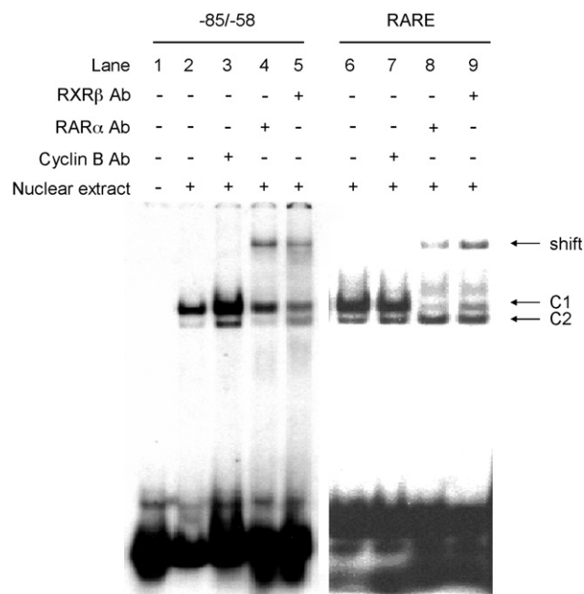
Fig. 4 – Binding of RARα to the mouse –82/–58 bp Raldh1 gene region. Nuclear extracts from Hepa-1 cells were incubated with radiolabeled –82/–58 bp (lanes 2–5), or radiolabeled consensus RARE (lanes 6–9), and then incubated with RARα antibody (Ab) (lanes 4 and 8), or RXRβ Ab (lanes 5 and 9) for 60 min. Lanes 3 and 7 were incubated with an unrelated Ab (Cyclin B). Arrows identify the shifted bands. A representative set of data from two independent experiments is shown.
